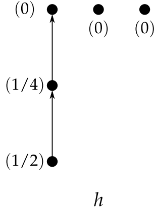
Figure 13: Calculating GRC_h .
