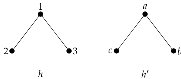
Figure 3: Relabeling.
